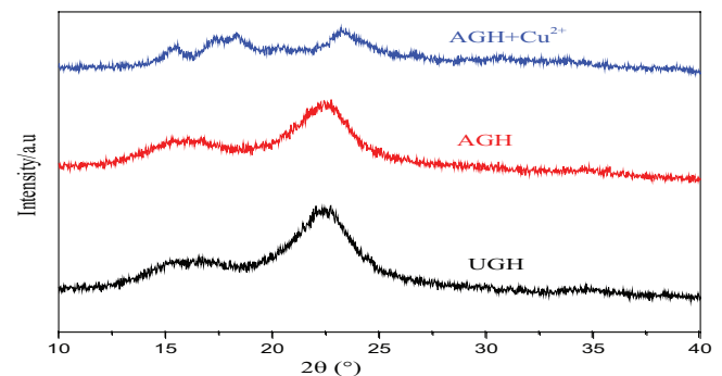
Fig. 2. XRD patterns of UGH, AGH, and AGH+Cu 2+ .
