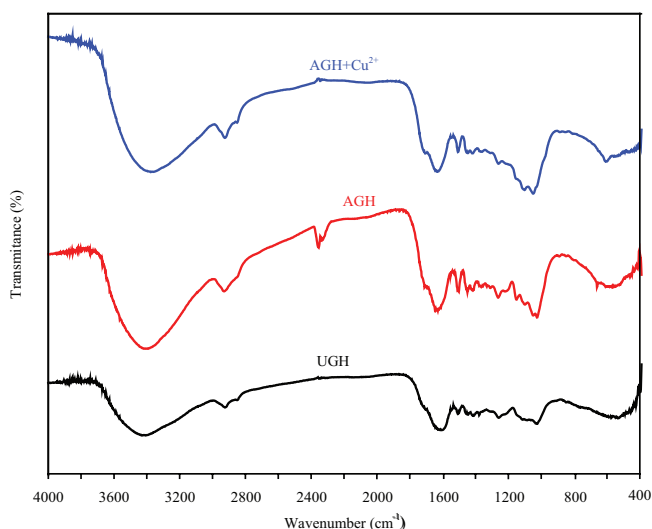
Fig. 1. The FTIR spectra of UGH, AGH, and AGH+Cu 2+ .
