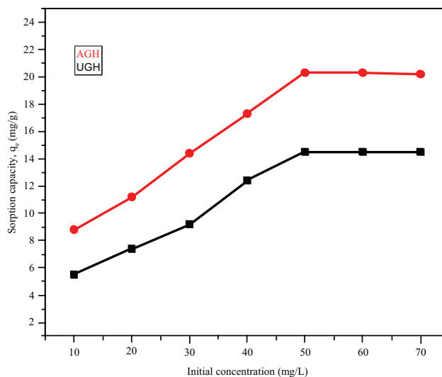
Fig. 5. Sorption capacity of Cu(II) ions against initial metal concentration by UGH and AGH at a pH of 5.0, contact time of 70 min and biomass dosage of 0.03 g.
