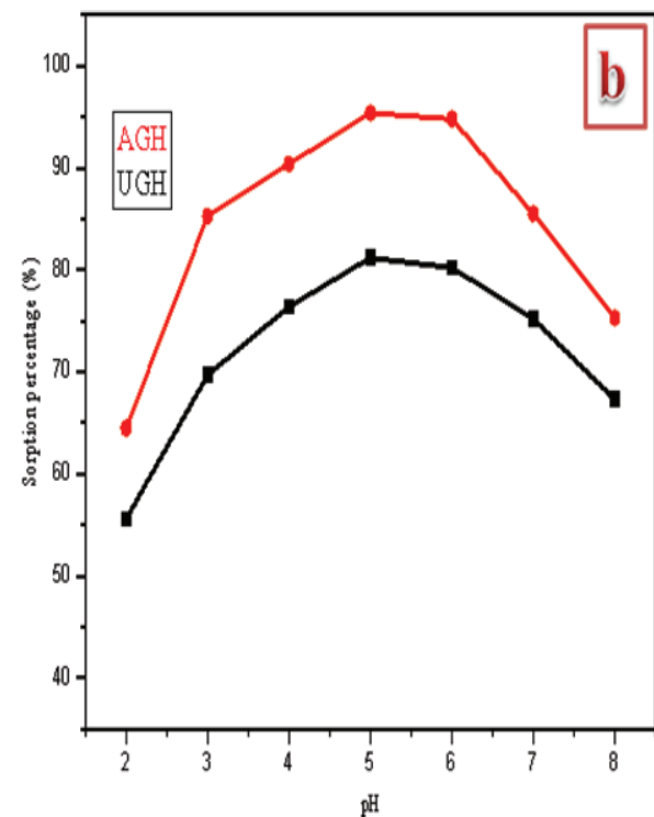
Fig. 8. Plots of (a) zeta potential and (b) sorption capacity of Cu(II) ions against pH by UGH and AGH at the initial metal concentration of 50 mg L -1 , a dosage of 0.03 g and contact time of 70 min.
