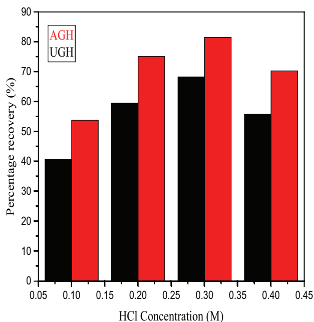
Fig. 12. Percentage recovery against different concentrations of a desorbing agent.
