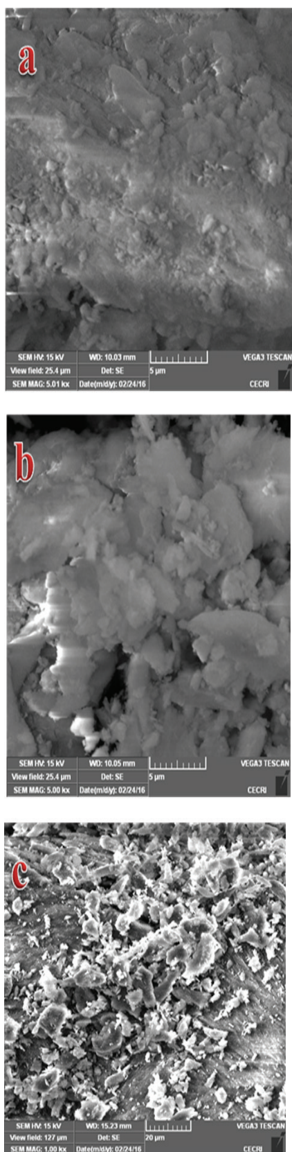
Fig. 4. SEM images of (a) unmodified groundnut husk, UGH, (b) acid-modified groundnut AGH, and (c) acid-modified groundnut +Cu 2+ .
