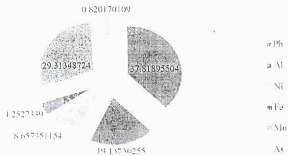
Figure 10. Pollution index percentage contributions by significant metals.
